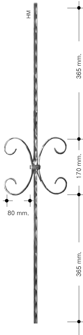
P-901 HM 1.437 kg.-3.167 lbs. Dim.170 x 900 mm. 6"11/16 x 35"7/16
