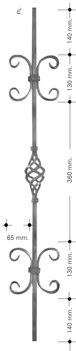
P-2401 1.900 kg.-4.188 lbs. Dim.150 x 900 mm. 5"7/8 x 35"7/16
