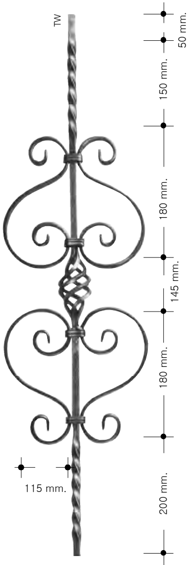
P-3301 TW 2.500 kg.-5.510 lbs. Dim.240 x 900 mm. 9"7/16 x 35"7/16
