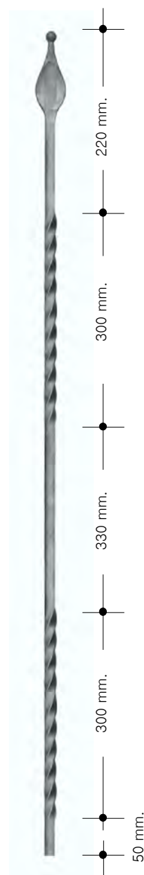
P-4305/B TW 1.356 kg.-2.988 lbs. Dim.40 x 1200 mm. 1"9/16 x 47"2/8
