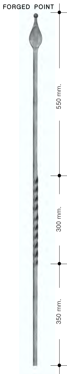
P-4305/A TW 1.356 kg.-2.988 lbs. Dim.40 x 1200 mm. 1"9/16 x 47"2/8
