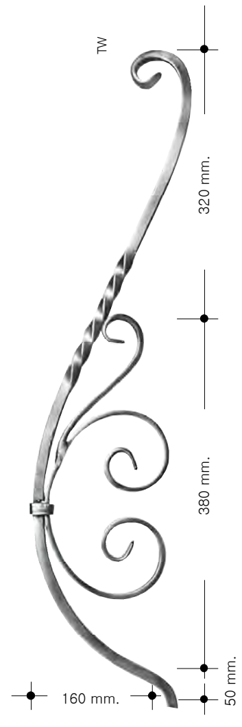
P-5105/B 1.560 kg.-3.438 lbs. Dim.160 x 750 mm. 2"5/16 x 29"4/8 Panel for last right and last left
