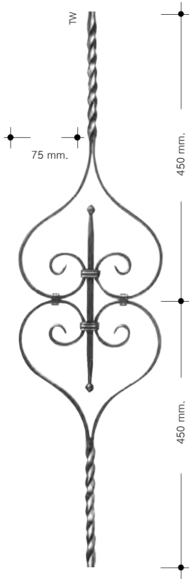
P-5001/D 2.030 kg.-4.474 lbs. Dim.160 x 900 mm. 2"5/16 x 35"7/16
