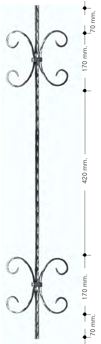
P-1001 1.848 kg.-4.073 lbs. Dim.170 x 900 mm. 6"11/16 x 35"7/16
