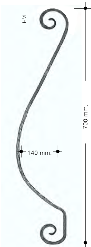
P-5105/C 1.045 kg.-2.303 lbs. Dim.160 x 750 mm. 2"5/16 x 29"4/8
