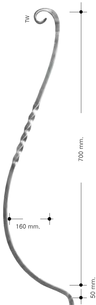
P-5105 1.045 kg.-2.303 lbs. Dim.160 x 750 mm. 2"5/16 x 29"4/8
