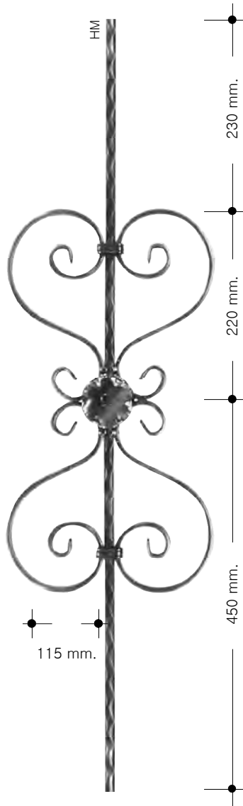
P-3401 HM 2.430 kg.-5.356 lbs. Dim.240 x 900 mm. 9"7/16 x 35"7/16
