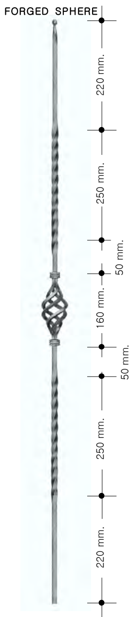
P-4105/B TW 1.410 kg.-3.107 lbs. Dim.55 x 1200 mm. 2"3/16 x 47"2/8
