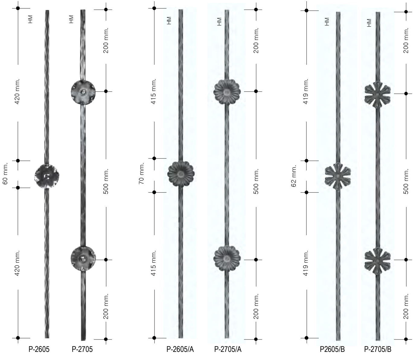
P-2605 HM 1.065 kg.-2.347 lbs. Dim.60 x 800 mm. 2"3/8 x 31"4/8
