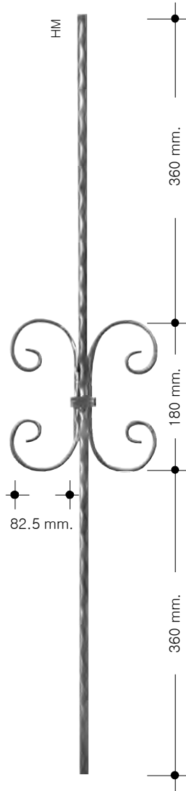
P-801 HM 1.590 kg.-3.504 lbs. Dim.175 x 900 mm. 6"7/8 x 35"7/16
