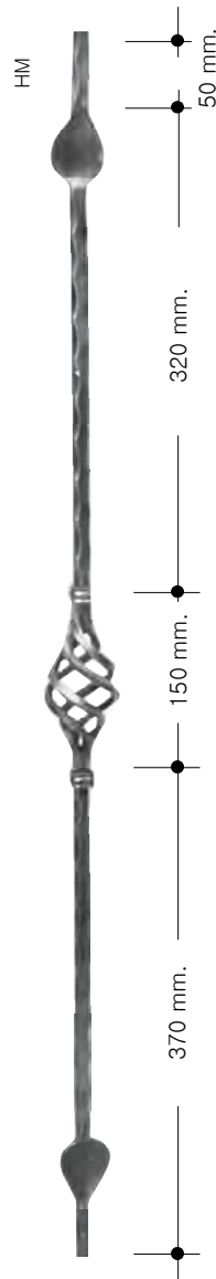
P-2505/A HM 1.125 kg.-2.480 lbs. Dim.55 x 900 mm. 12"1/8 x 5"2/8
