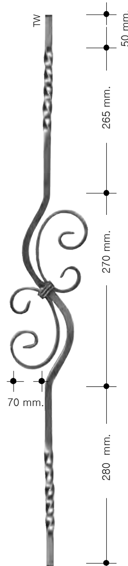
P-3001TW 1.530 kg.-3.372 lbs. Dim.130 x 900 mm. 5"1/8 x 35"7/16
