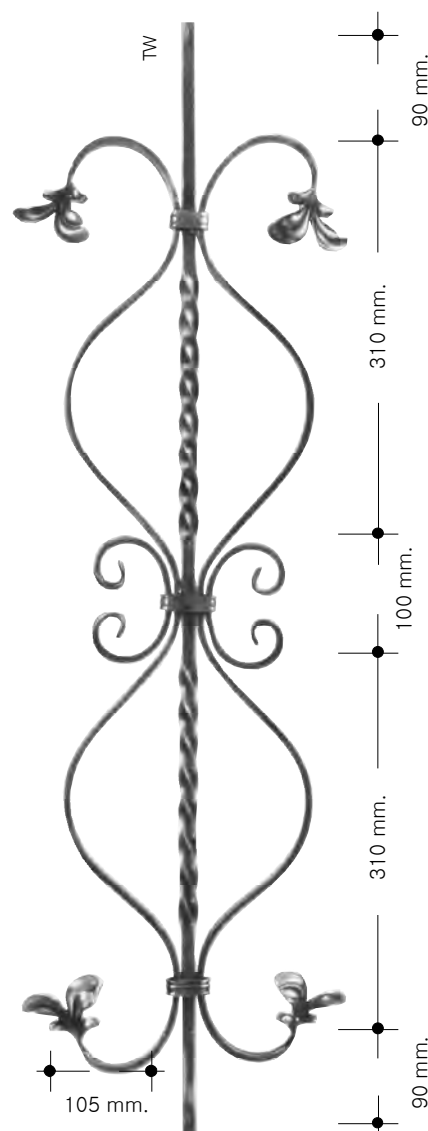
P-3601 TW 2.660 kg.-5.863 lbs. Dim.195 x 900 mm. 7"11/16 x 35"7/16
