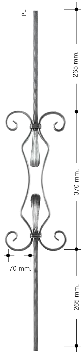
P-2001 HM 1.670 kg.-3.681 lbs. Dim.150 x 900 mm. 5 7 / 8 x 35 7 / 16
