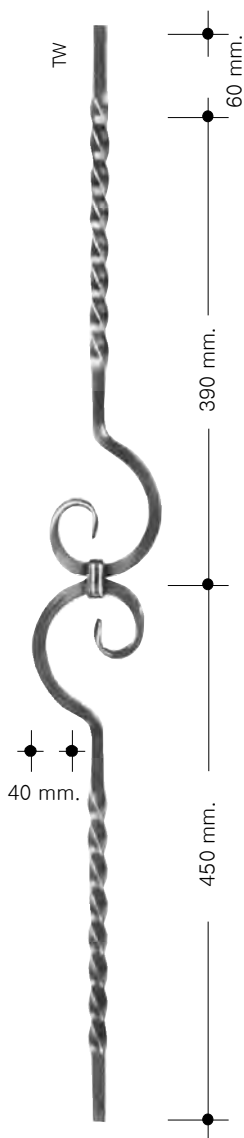
P-1805 TW 1.375 kg.-3.031 lbs. Dim.90 x 900 mm. 3 9 / 16 x 35 7 / 16
