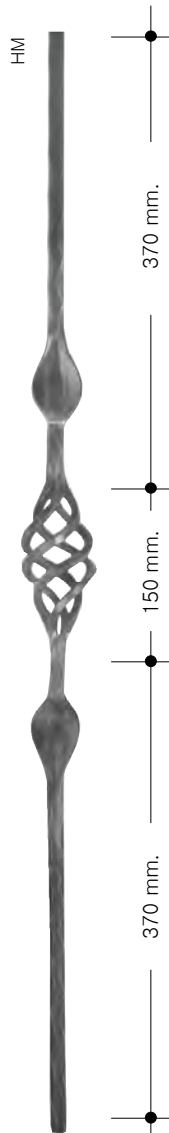
P-2505 HM 1.088 kg.-2.398 lbs. Dim.55 x 900 mm. 12"1/8 x 5"2/8
